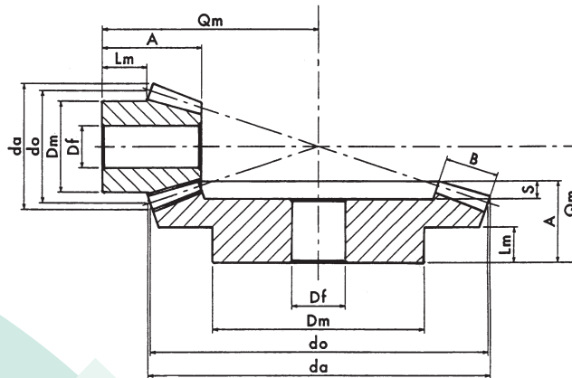
MATERIAL: C 43 STEEL – UNI 7847
